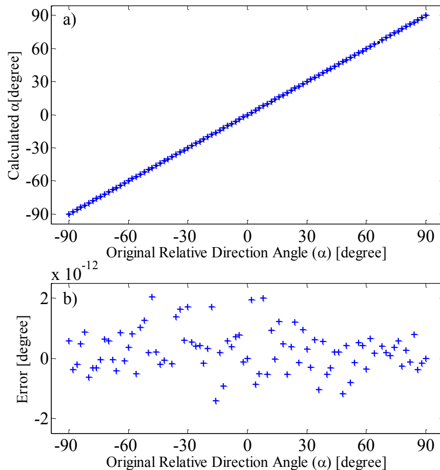
Figure 4.2 \alpha angles calculated from pinhole model and their error to ground truth; a) the original angles with black dots (covered by calculated angles) and the calculated angles with blue plus signs; b) the error for each calculated angle
