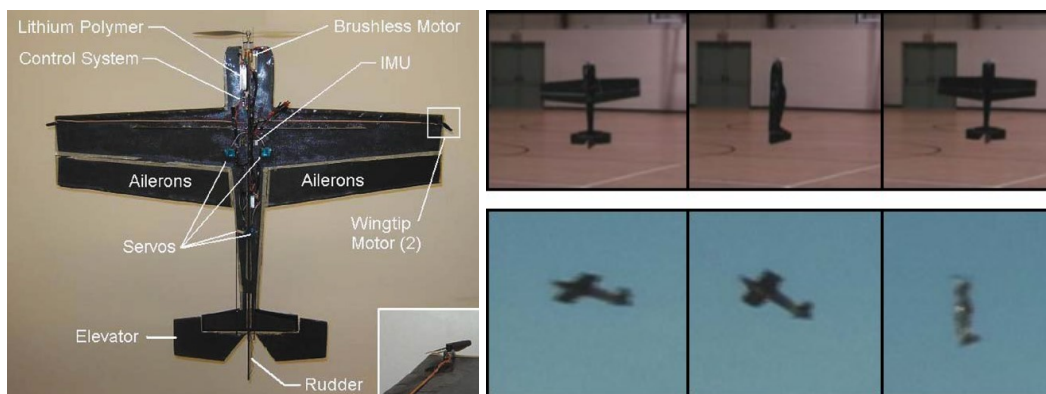
Figure 2.8 Fixed-wing MAV with hovering capability and OF based collision avoidance, autonomous hover and transition from cruise to hover
