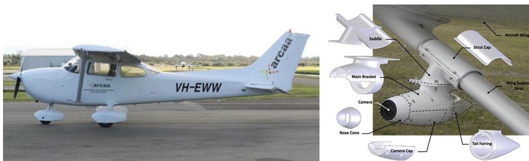
Figure 2.11 Modified Cessna 172 aircraft and the used camera frame
