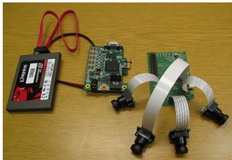
Figure 7.3 The image capturing, processing, and storing system; Diagram of the components (upper). The physical hardware components (lower) [12]
