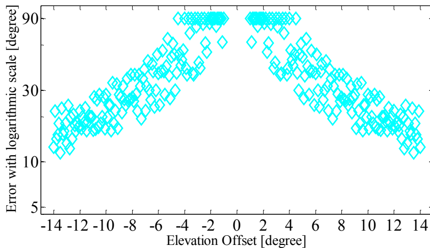
Figure 4.8 Maximum of absolute value of the errors of the rounded \alpha angles calculated with pinhole camera model in different positions and from 2 km distance along the X axis; on the horizontal axis the elevation offset; on the vertical axis the error in degree with logarithmic scale
