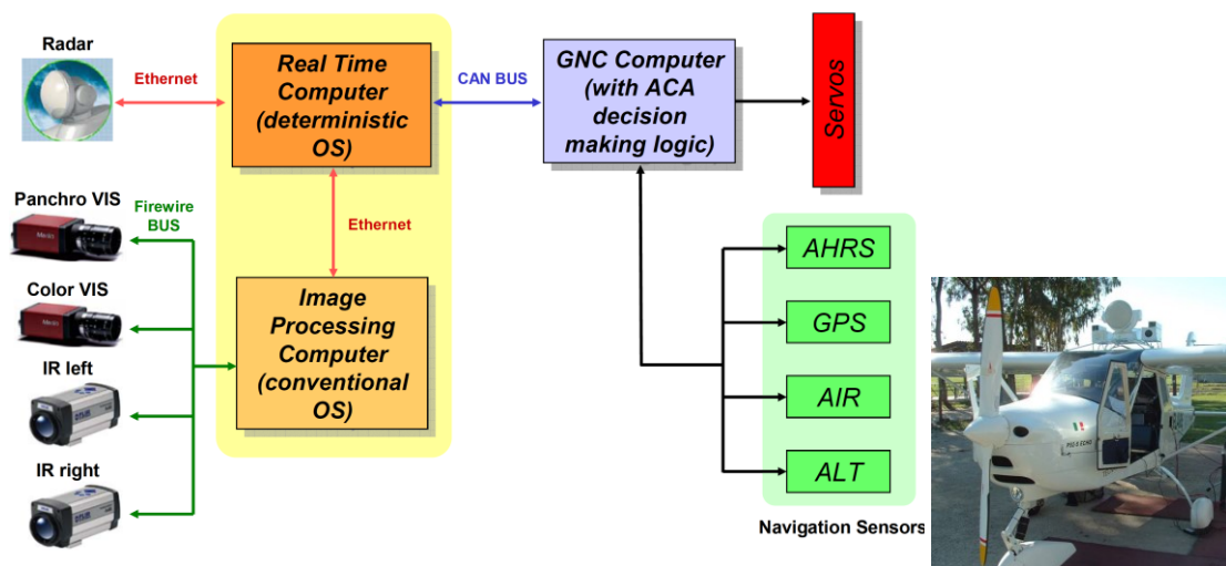
Figure 2.5 Multi-sensor-based fully autonomous non-cooperative collision avoidance system and the system placed to TECNAM P-92
